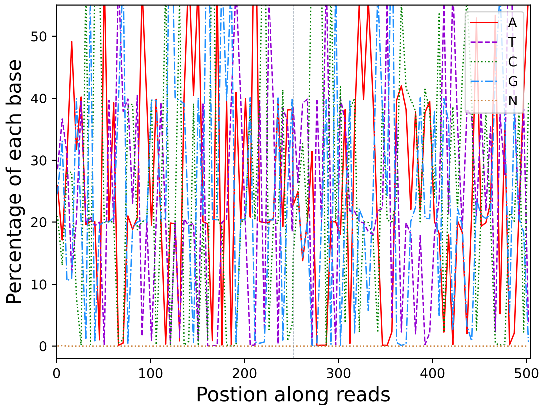
Base percentage along reads (R10322)
